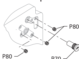
View "A" with pressure limiter port A, HPRV port B, right hand rotation (B)
