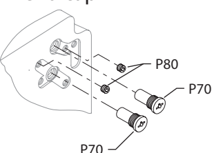
View "A" with pressure limiters, left hand rotation, (1, 5 & 6)
