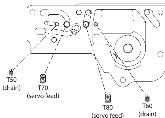
Possible orifice locations
