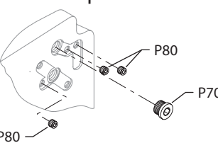
View "A" without pressure limiters, left/right hand rotation (2 & 7)
