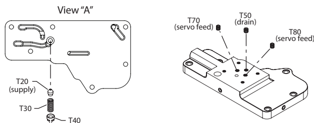
Possible orifice locations
