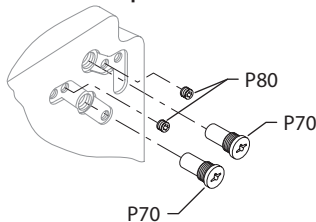
View "A" with pressure limiters, left hand rotation, (1, 5 & 6)
