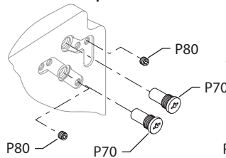
View "A" with pressure limiters, right hand rotation, (1, 5 & 6)
