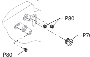
View "A" without pressure limiters, left/right hand rotation (2 & 7)
